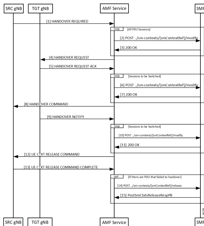
Figure 1: N2 Handover without AMF Change Call Flow
