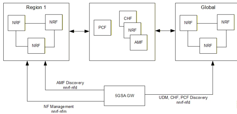
Figure 15: NRF Deployment
