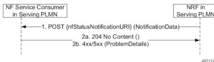
Figure 9: NFStatus Notify Call Flow
