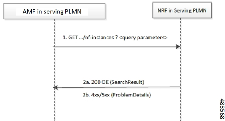
Figure 12: Service Discovery Request Call Flow
