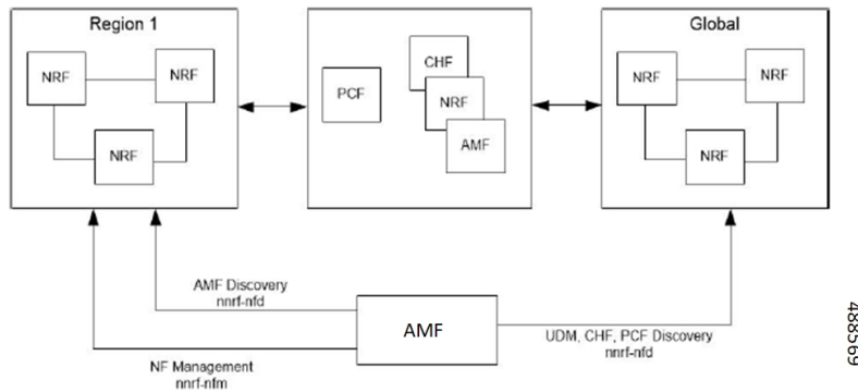
Figure 15: NRF Deployment
