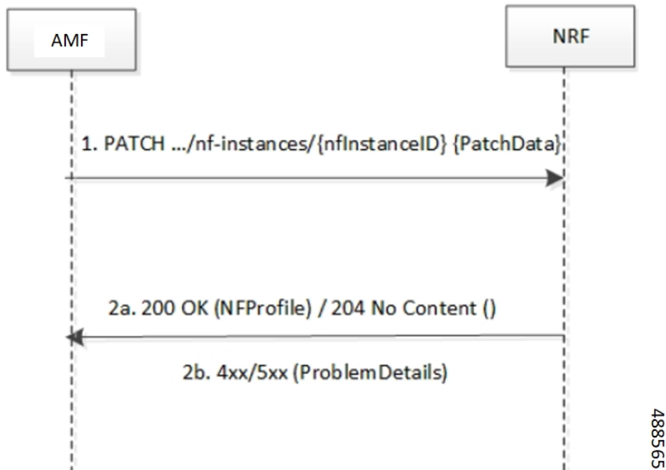
Figure 5: NF Heartbeat Call Flow
