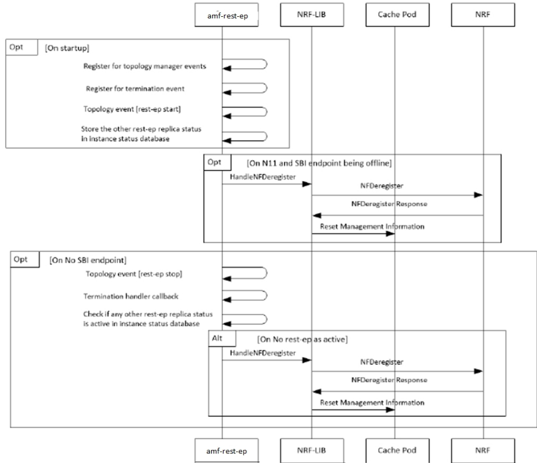
Figure 3: NF Deregistration Trigger Events Call Flow
