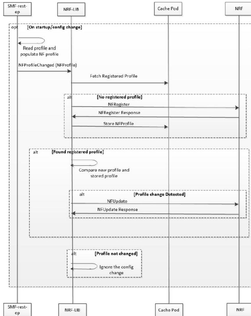
Figure 11: NF Registration and NF Update Call Flow
