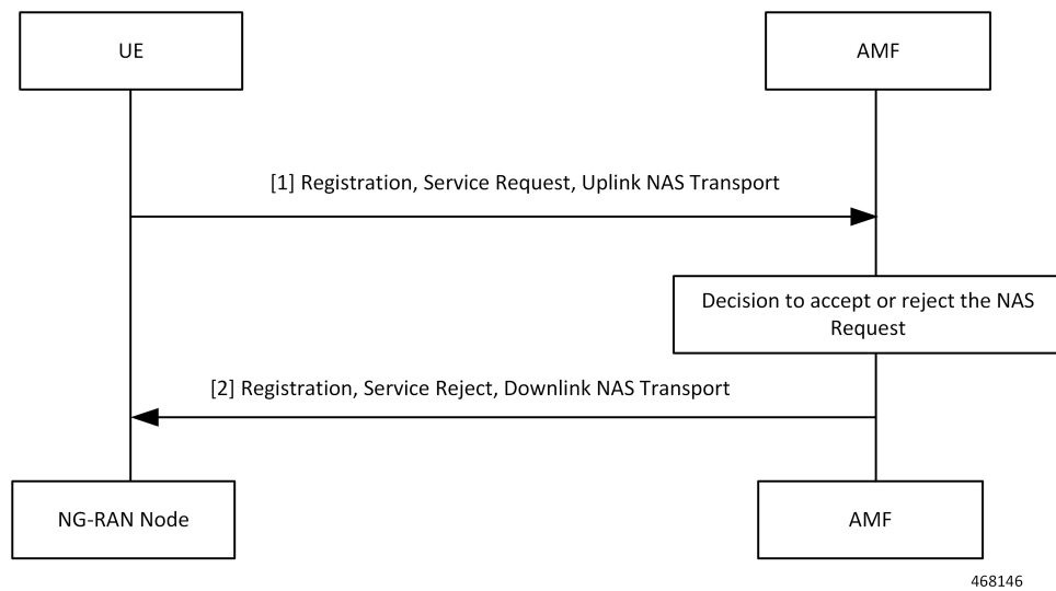
Figure 3: NAS Congestion Control Call Flow
