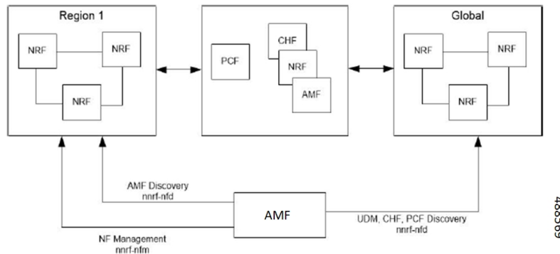
Figure 10: NRF Deployment
