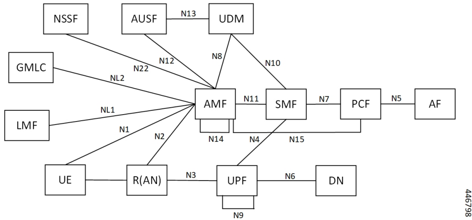
Figure 9: Interfaces
