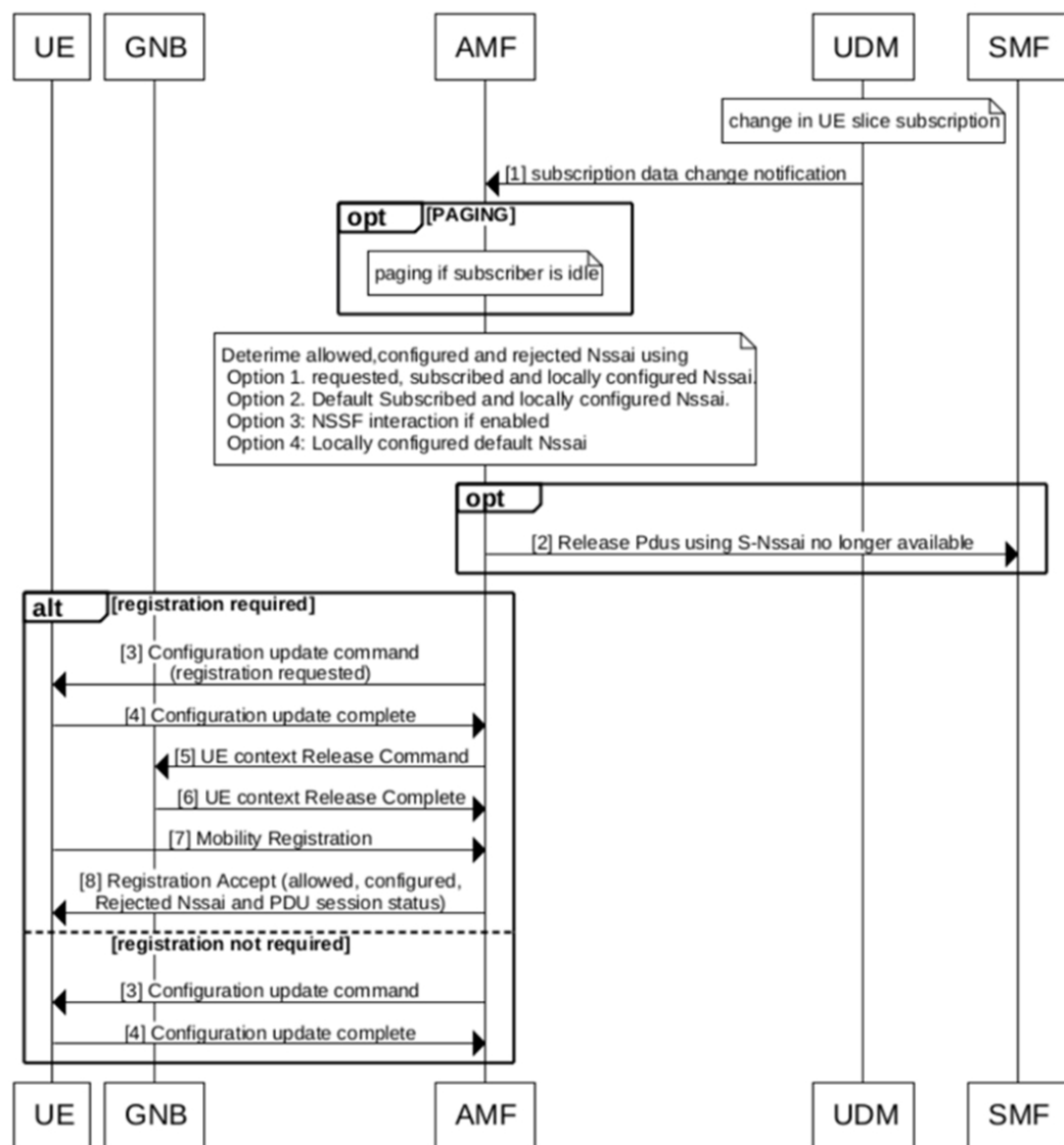
Figure 52: UE Configuration Update for UDM Subscription Change
