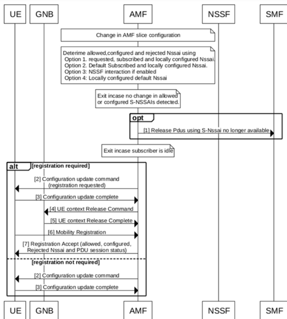
Figure 54: Slice Configuration Change
