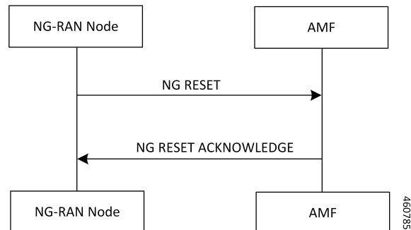
Figure 53: Reset Procedure Initiated from gNB to AMF
