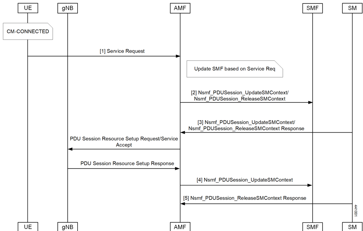
Figure 62: Connected Mode Call Flow
