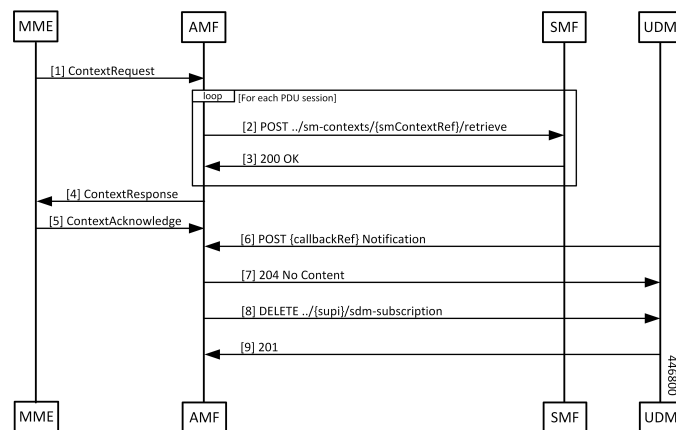
Figure 40: AMF to MME Idle Mode Handoff Call Flow
