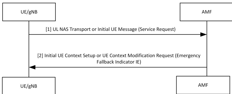
Figure 86: Service Request Procedure Call Flow
