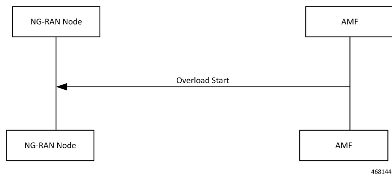
Figure 51: Overload Start Message Call Flow
