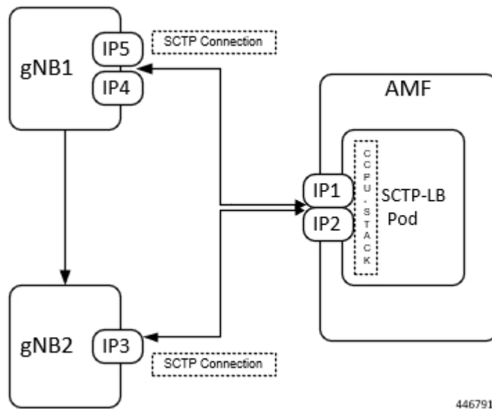
Figure 61: SCTP Multihoming Support
