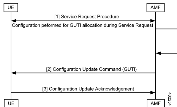
Figure 73: Sending the New GUTI to UE Call Flow
