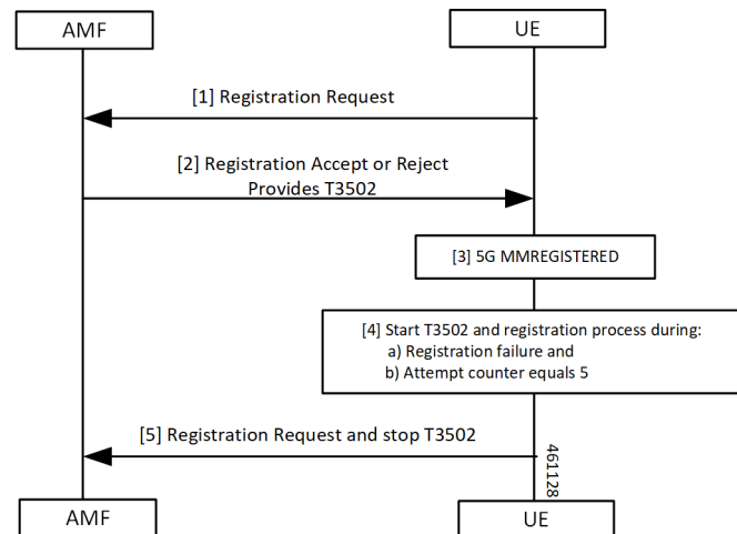
Figure 60: T3502 Timer Call Flow
