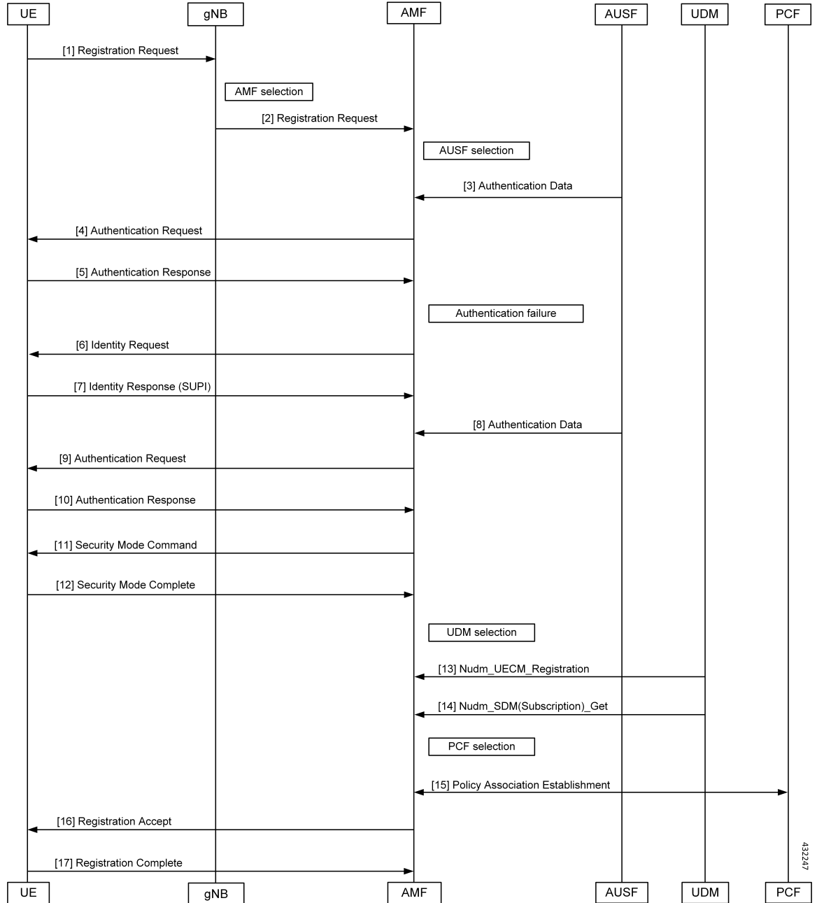
Figure 13: UE Identity Procedure for Authentication Failure Call Flow
