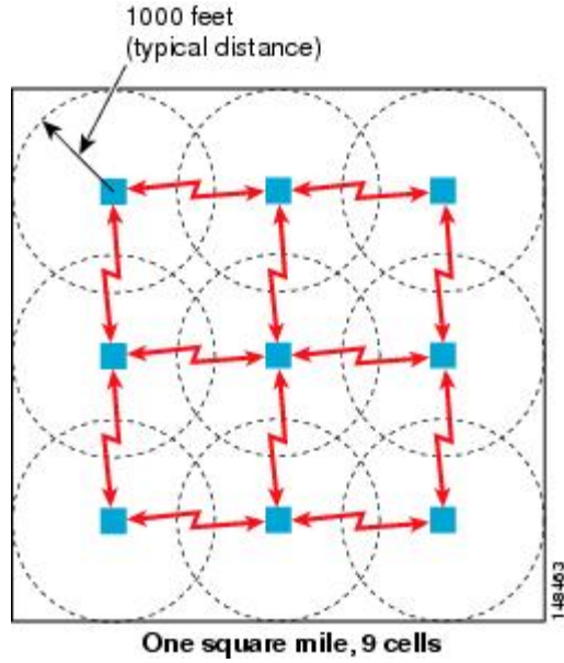
Figure 7: Path Loss Exponent 2.3 to 2.7
