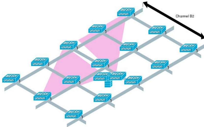
Figure 19: Two RAPs per Cell on Different Channels
