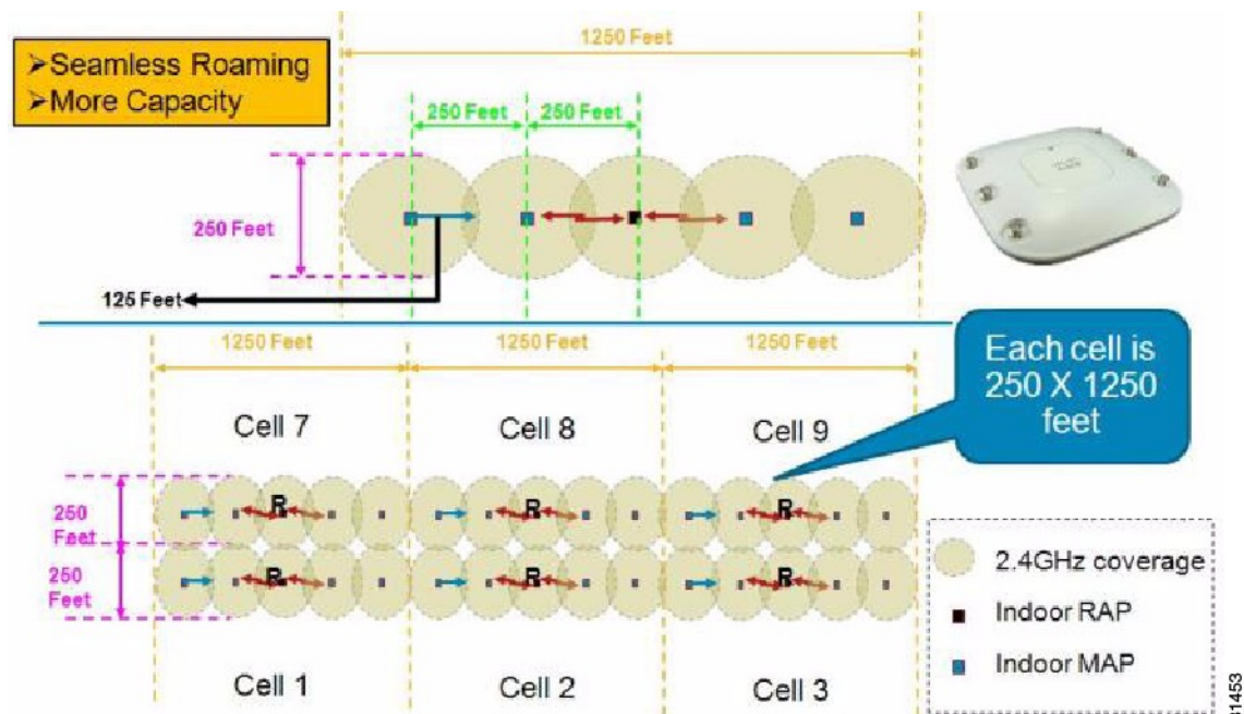
Figure 16: Cell Radius of 125 Feet (38 meters) and Access Point Placement for Indoor 11n Mesh Networks
