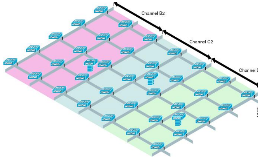
Figure 12: Multiple RAP and MAP Cells
