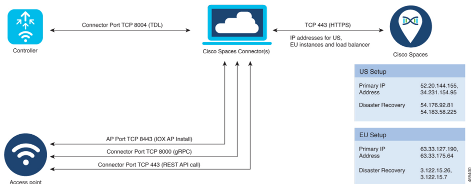
Figure 3: IoT Services
