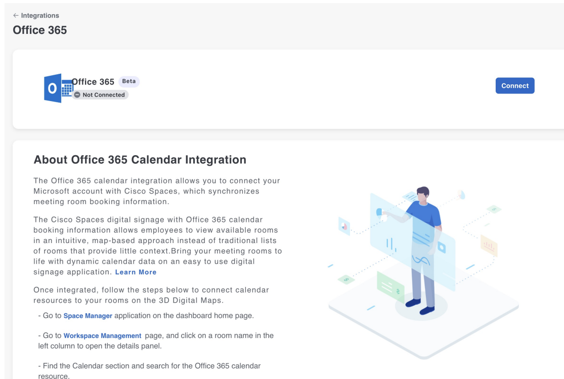
Figure 2: Office 365 Integrations
