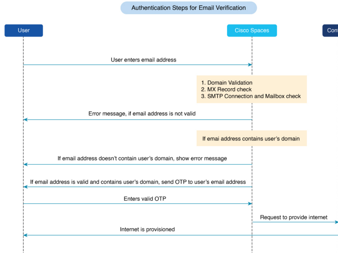
Figure 3: Authentication Workflow
