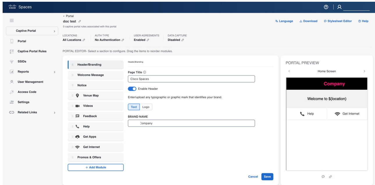
Figure 2: Header/Branding Module
