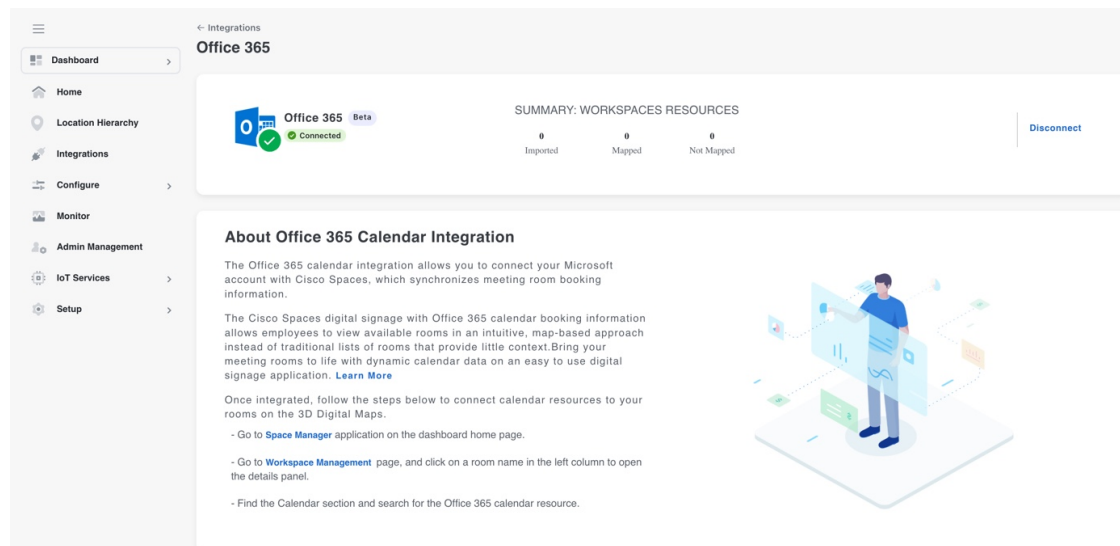
Figure 2: Office 365 Integrations
