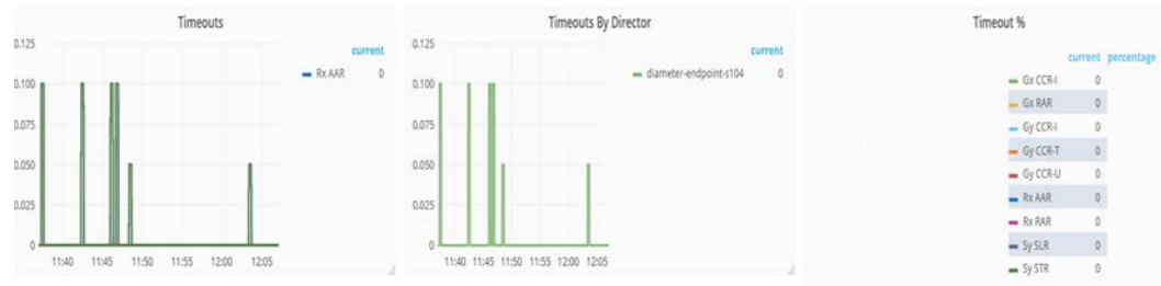
Figure 9: Database Queries
