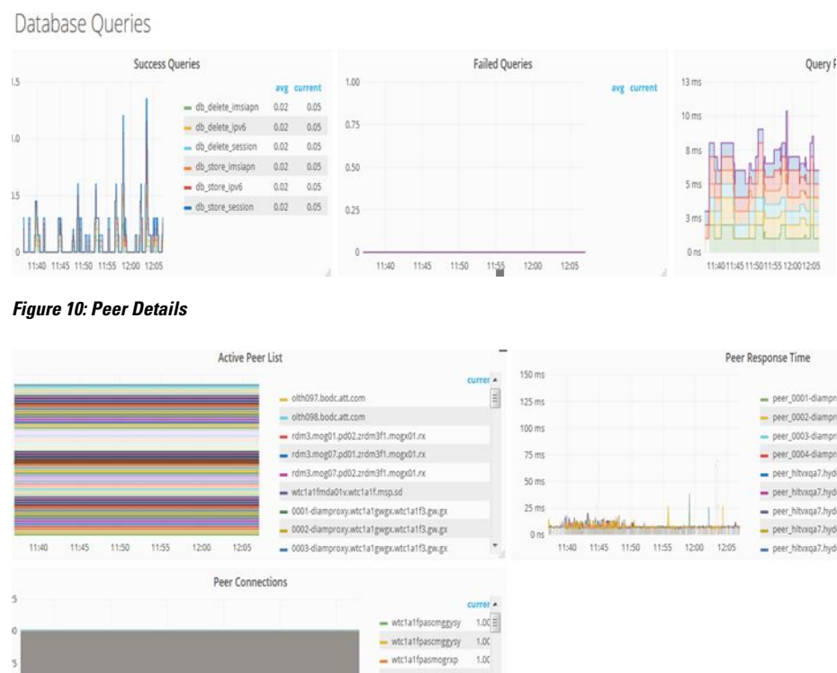
Figure 10: Peer Details
