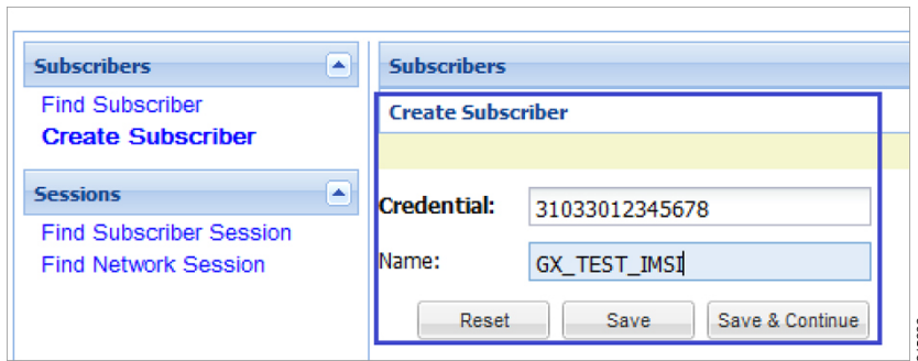
Figure 3: Create Subscriber
