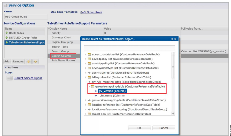
Figure 12: Search Column Mapping
