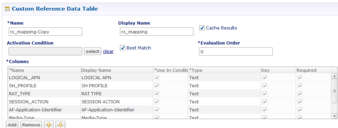
Figure 14: Best Match Option
