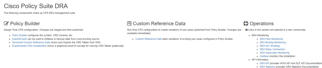
Figure 20: Main Page
