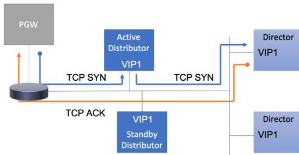
Figure 8: Direct Routing
