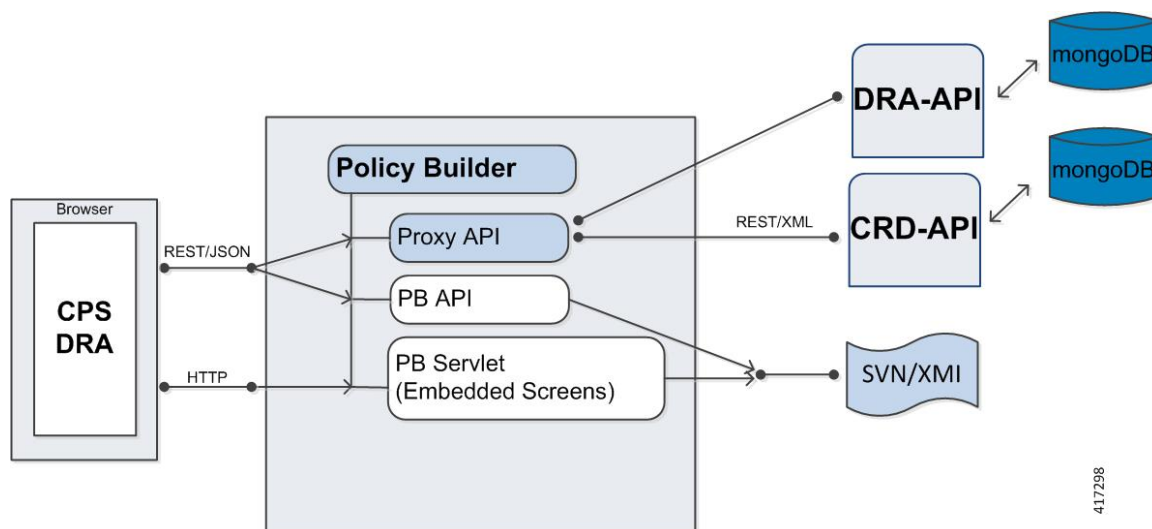
Figure 1: DRA Architecture
