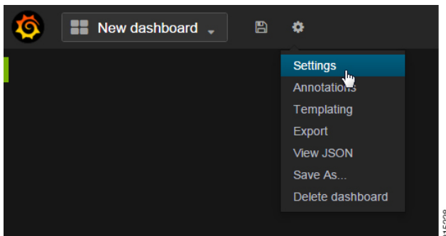
Figure 35: Settings
