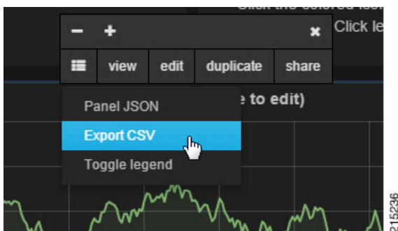
Figure 53: Export
