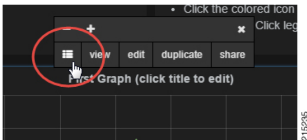
Figure 52: Rows
