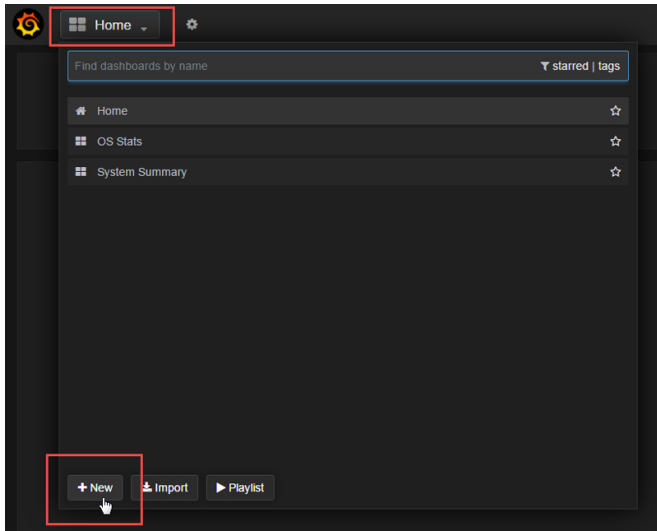
Figure 32: Home
