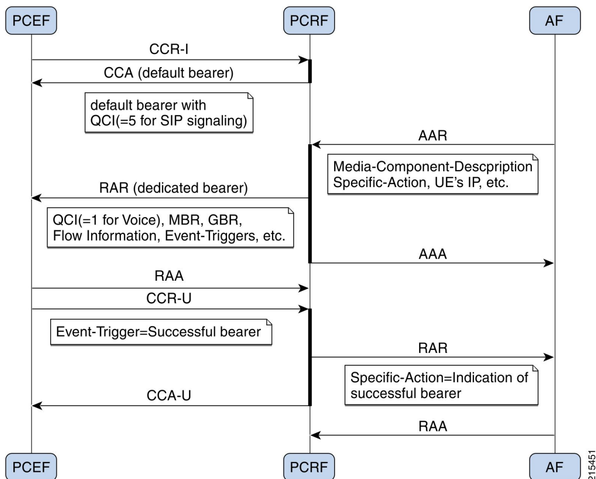
Figure 1: Example VoLTE Call
