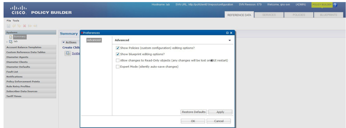
Figure 6: Preferences - Blueprints 2
