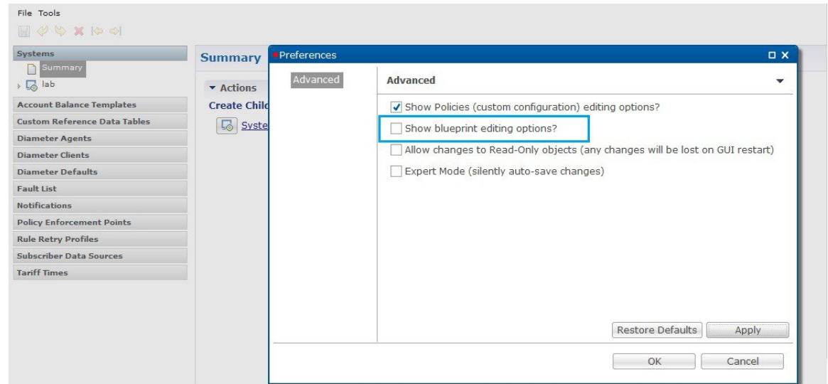
Figure 6: Preferences - Blueprints 2
