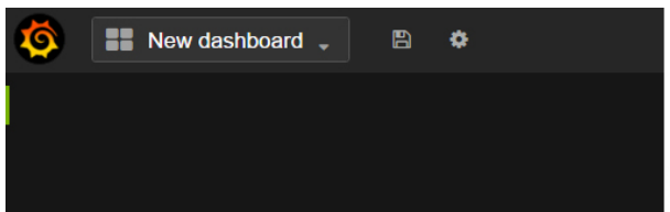
Figure 17: Blank Dashboard
