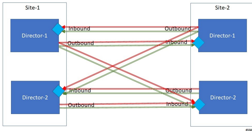
Figure 13: Priority-based Relay Routing Flow
