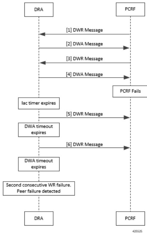
Figure 49: vDRA Peer Detection Failure
