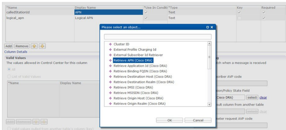
Figure 72: Adding AVPs
