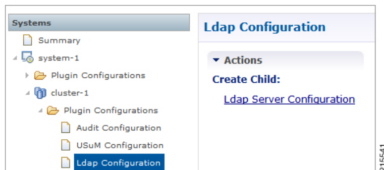
Figure 14: LDAP Configuration
