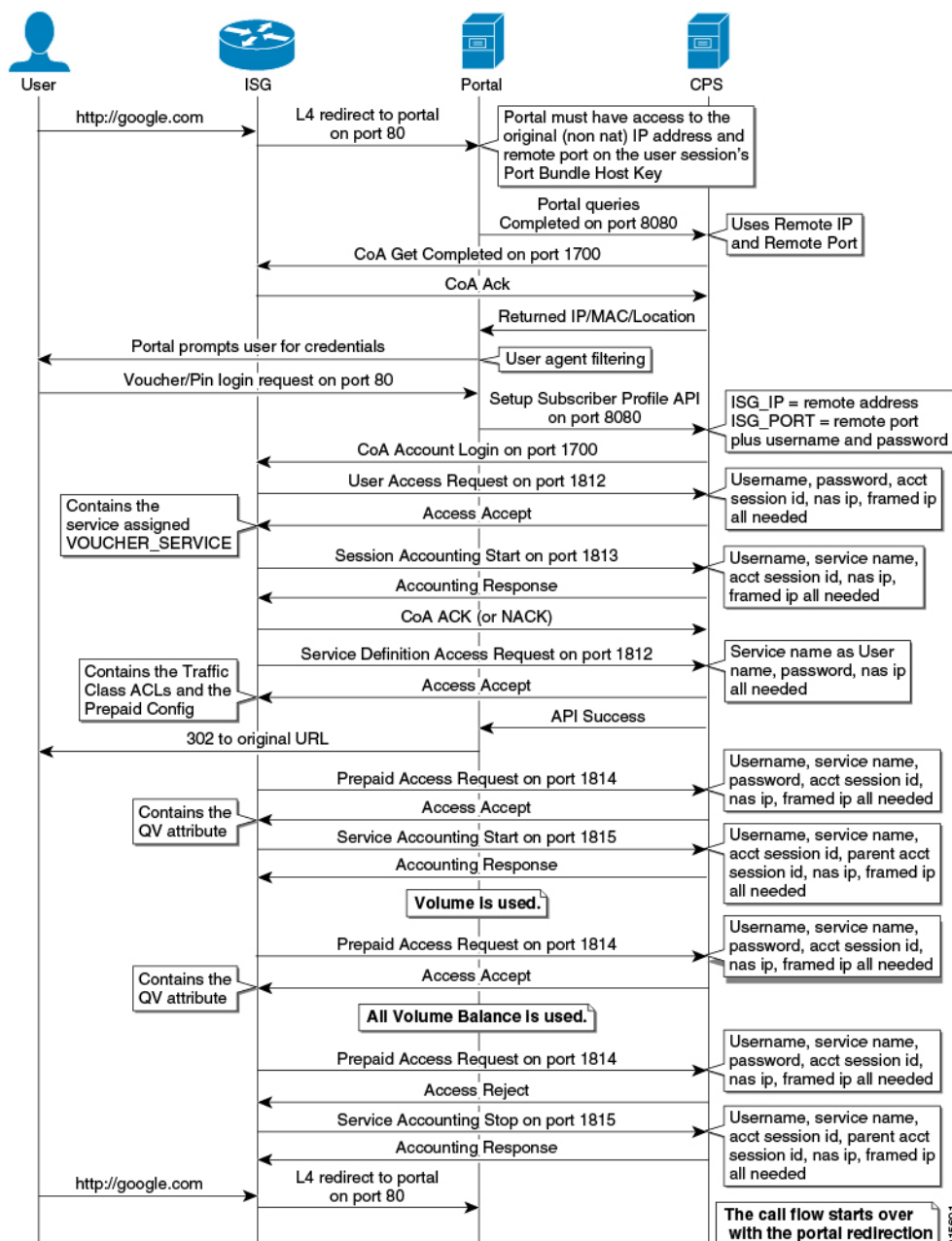
Figure 1: One-Click Call Flow
