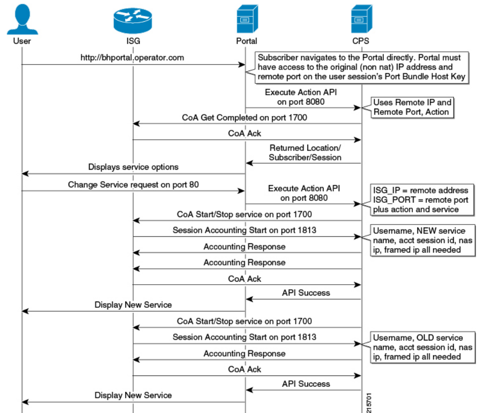
Figure 6: Service Selection Call Flow
