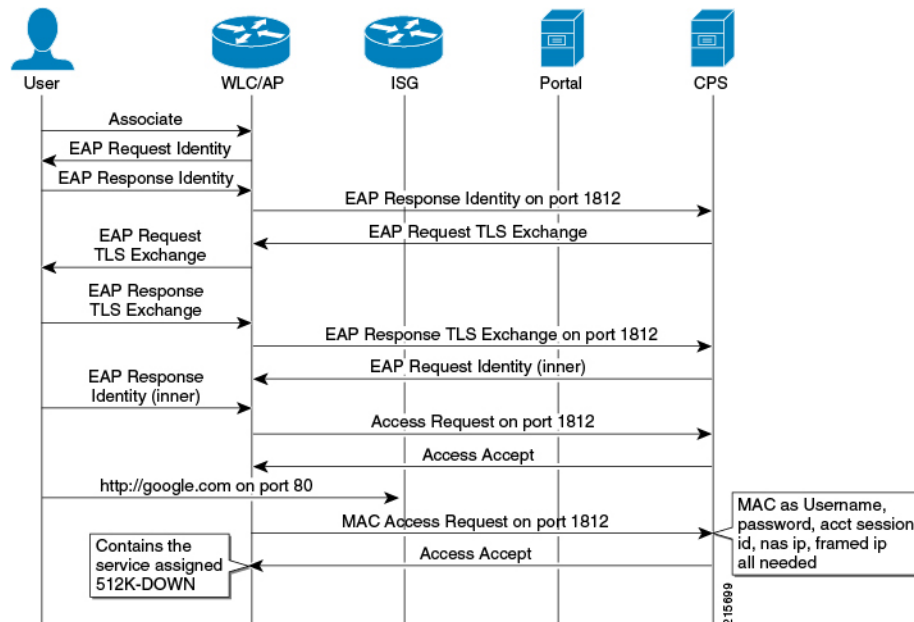
Figure 5: EAP-TTLS Call Flow
