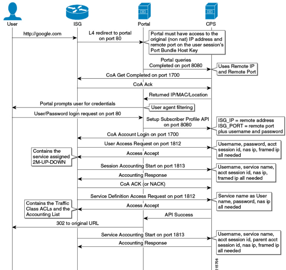
Figure 8: Tiered Services Call Flow
