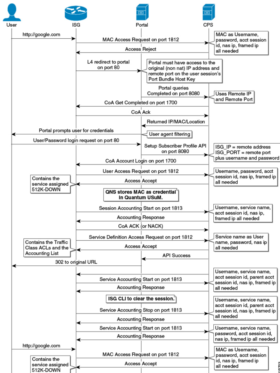
Figure 7: MAC TAL Call Flow
