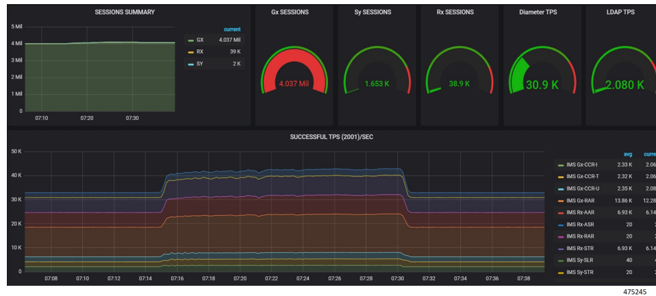
Figure 4: Grafana Graph
