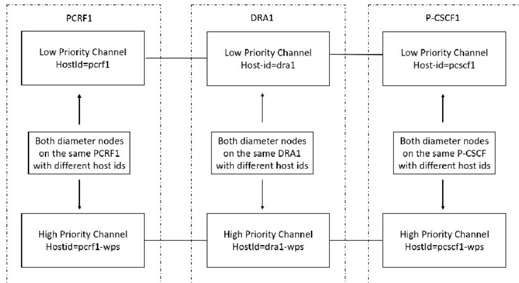
Figure 134: High-Level Overview of Low and High Priority Channels over Rx Interface
