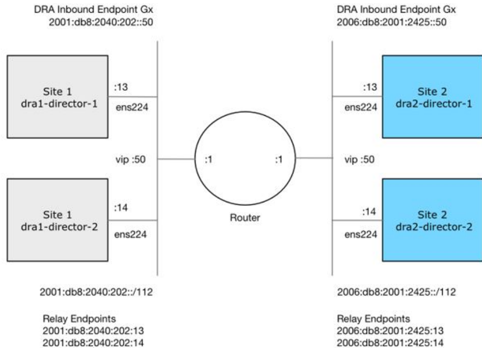
Figure 57: Example of Relay Endpoints
