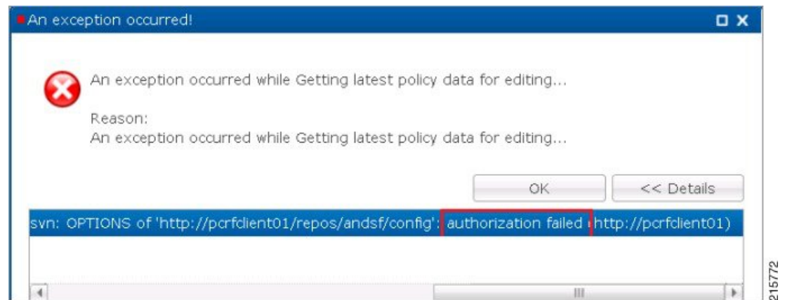
Figure 19: Exception Occurred
