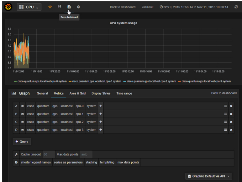
Figure 42: Save
