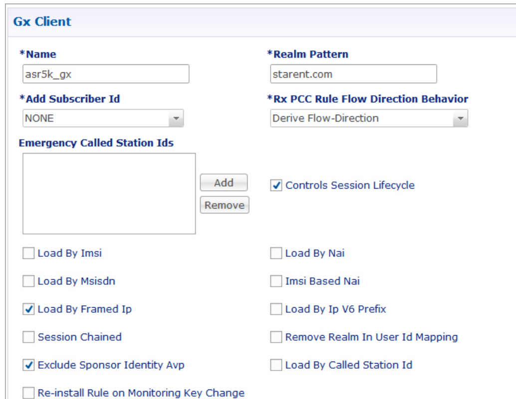
Figure 21: Excluding Sponsor-Identity AVP
