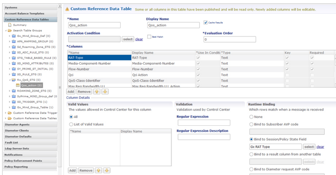
Figure 11: Search Table Group
