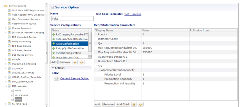
Figure 5: RxQoSInfomration Service
