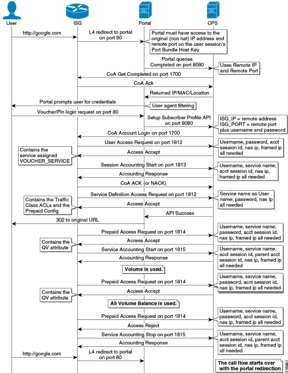
Figure 1: One-Click Call Flow
