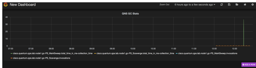
Figure 32: Example Graph
