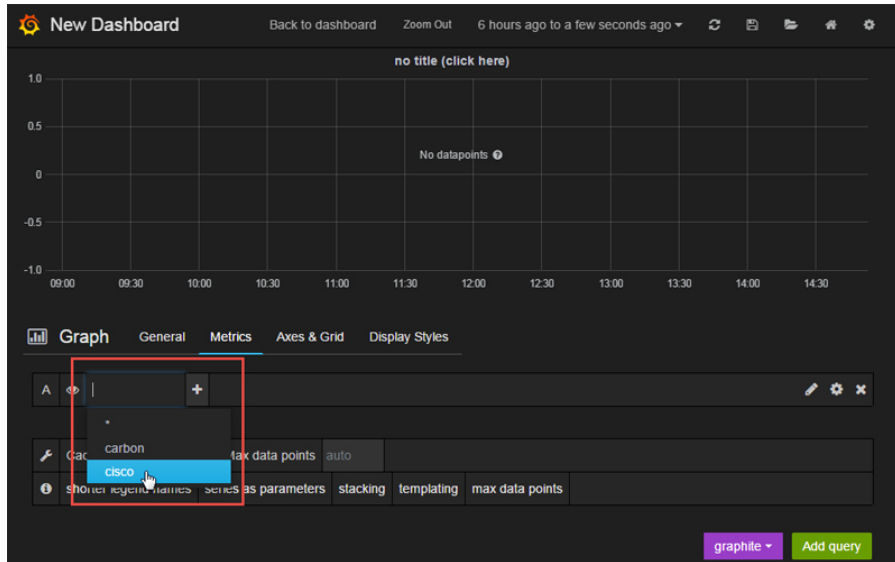
Figure 39: Metric Selection
