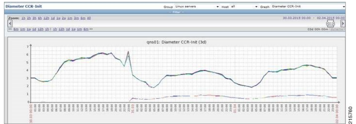
Figure 4: Zabbix Graph
