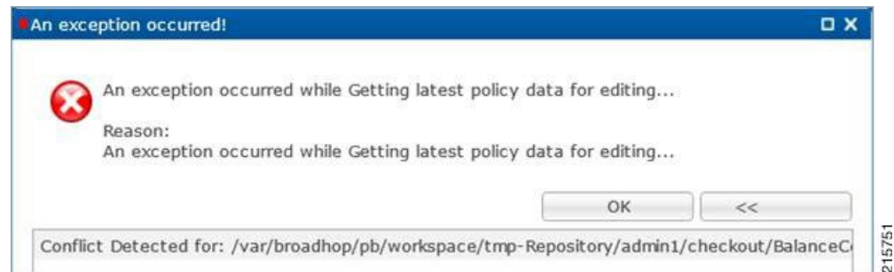
Figure 16: Login Error
