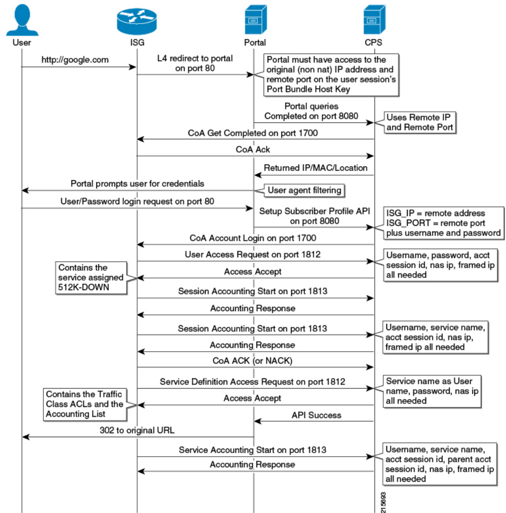
Figure 2: User/Password Login Call Flow
