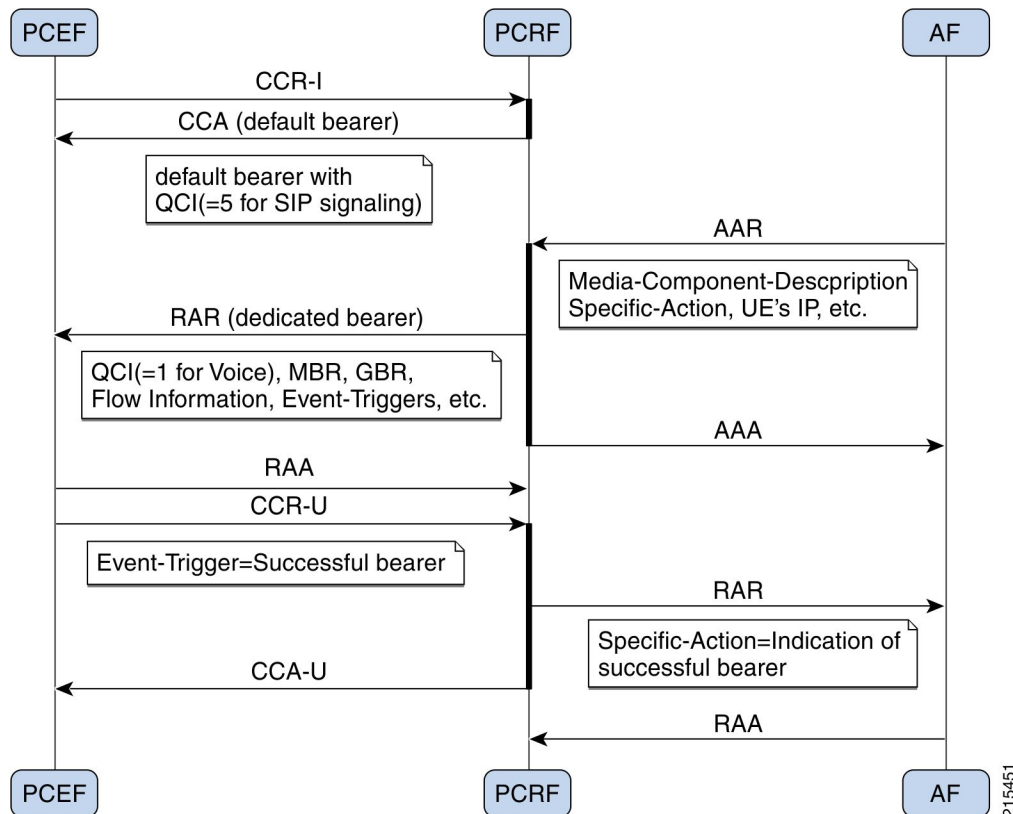
Figure 1: Example VoLTE Call
