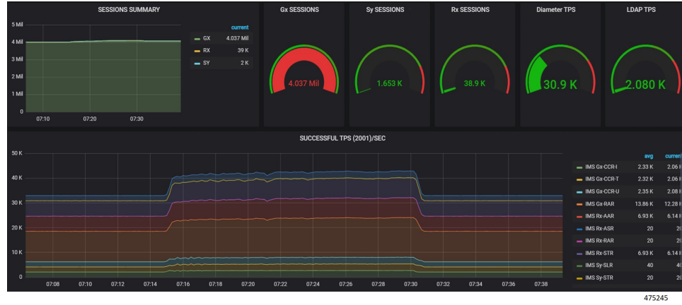
Figure 4: Grafana Graph
