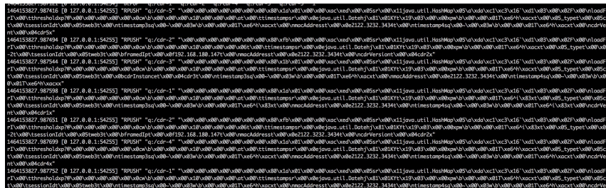
Figure 27: REDIS Output
