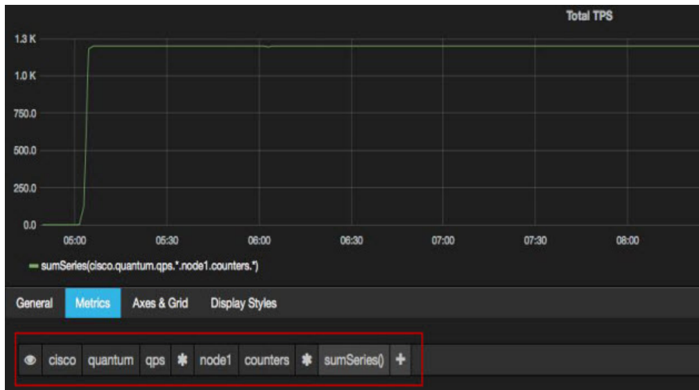
Figure 30: Total TPS
