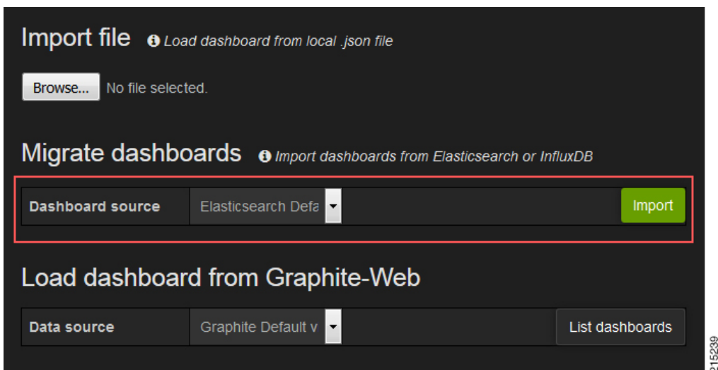
Figure 15: Import File
