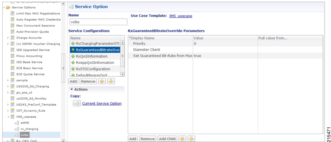
Figure 7: RxGuaranteedBitrateOverride Service
