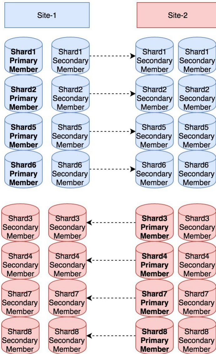
Figure 21: Failover Scenario
