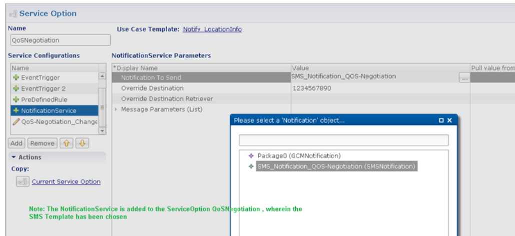
Figure 10: Notification Object
