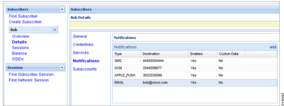
Figure 16: Notification Destinations
