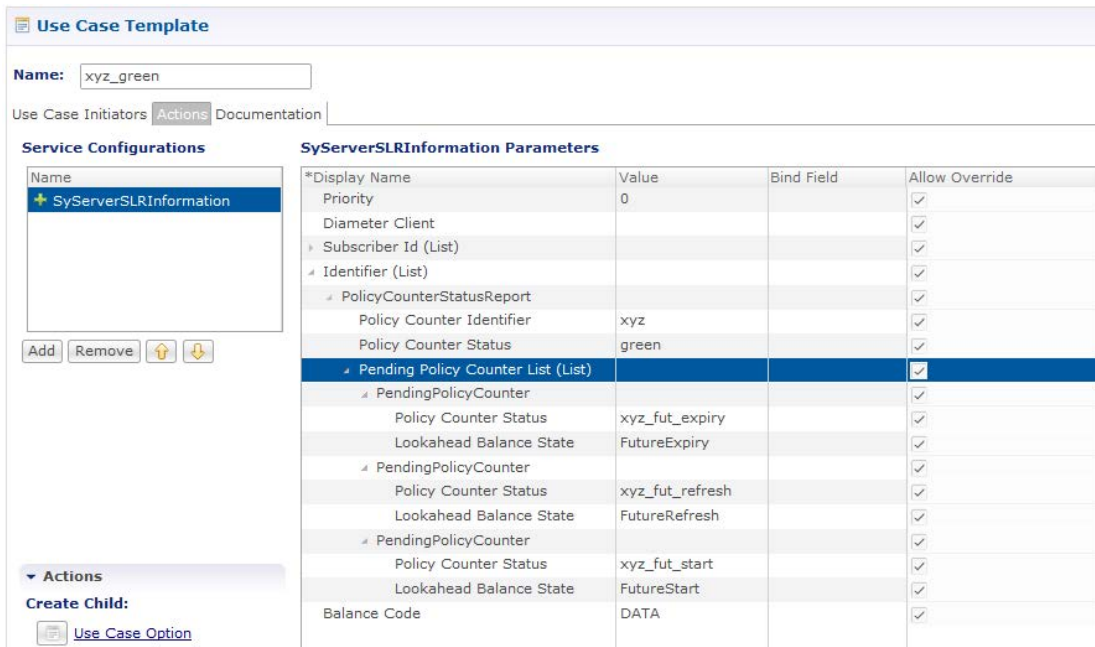
Figure 8: SyServerSLRInformation Service Configuration Object
