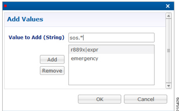
Figure 15: Add Values
