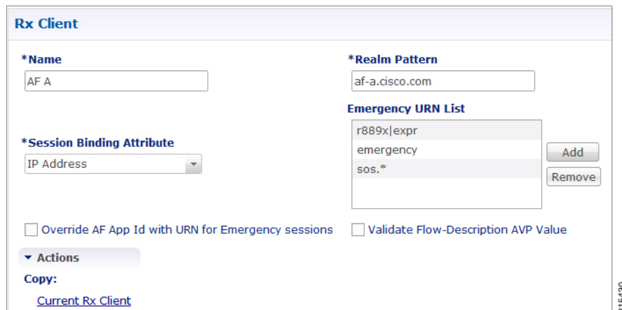
Figure 16: Add/Remove URN
