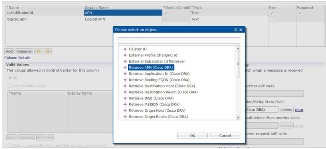
Figure 24: Adding AVPs
