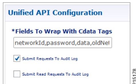
Figure 8: Unified API Configuration
