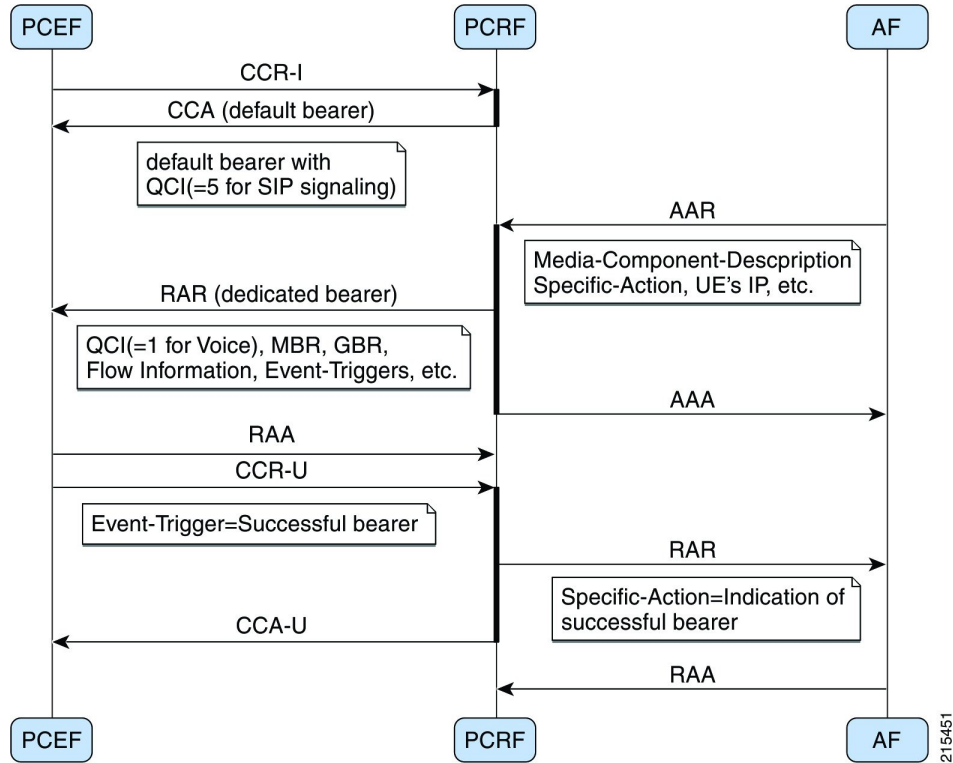
Figure 1: Example VoLTE Call
