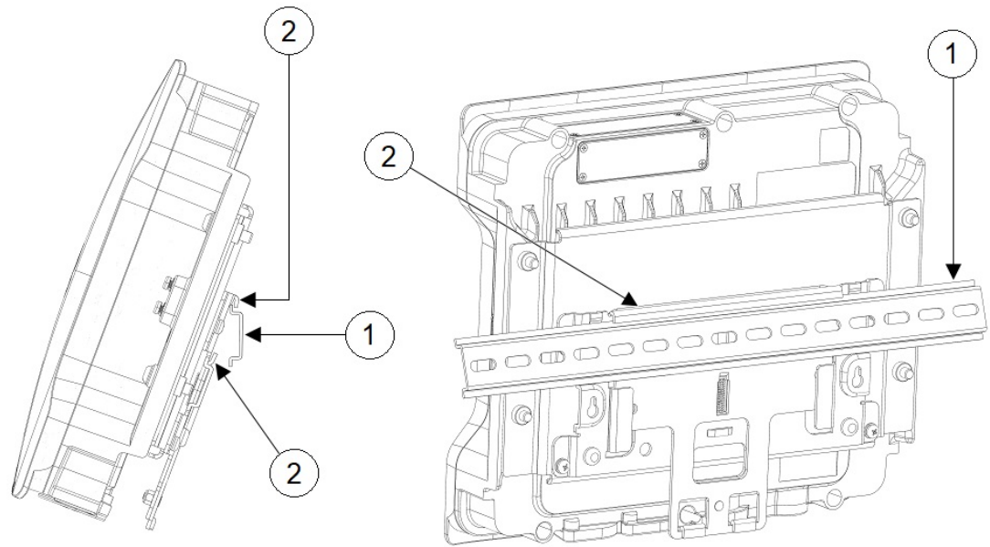
Figure 1: DIN Rail Mounting Assembly
