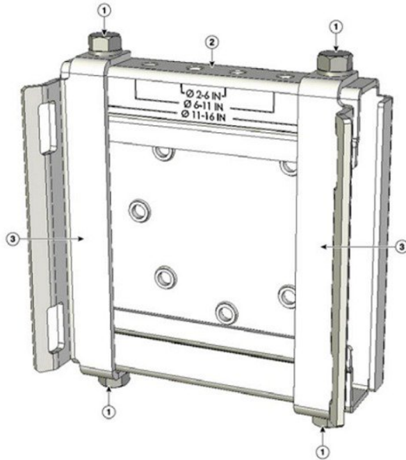
Figure 3: Assembled Pole Clamp Bracket and Strap Brackets
