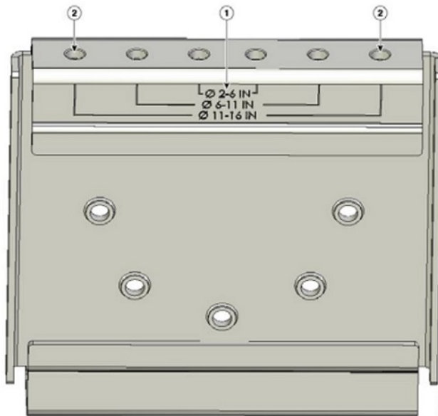
Figure 2: Pole Clamp Bracket Adjustment Hole Locations
