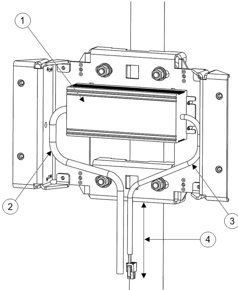
Figure 7: Power Adapter Installed Using Mounting Bracket AIR-ACCPMK3700-2=
