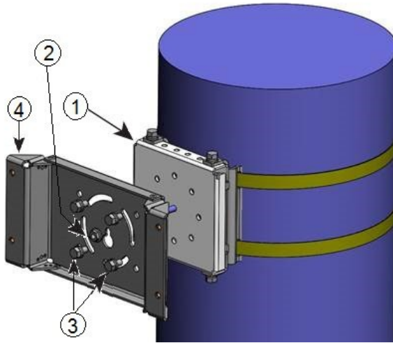
Figure 5: Mounting Bracket and Pole Clamp Bracket Assembly
