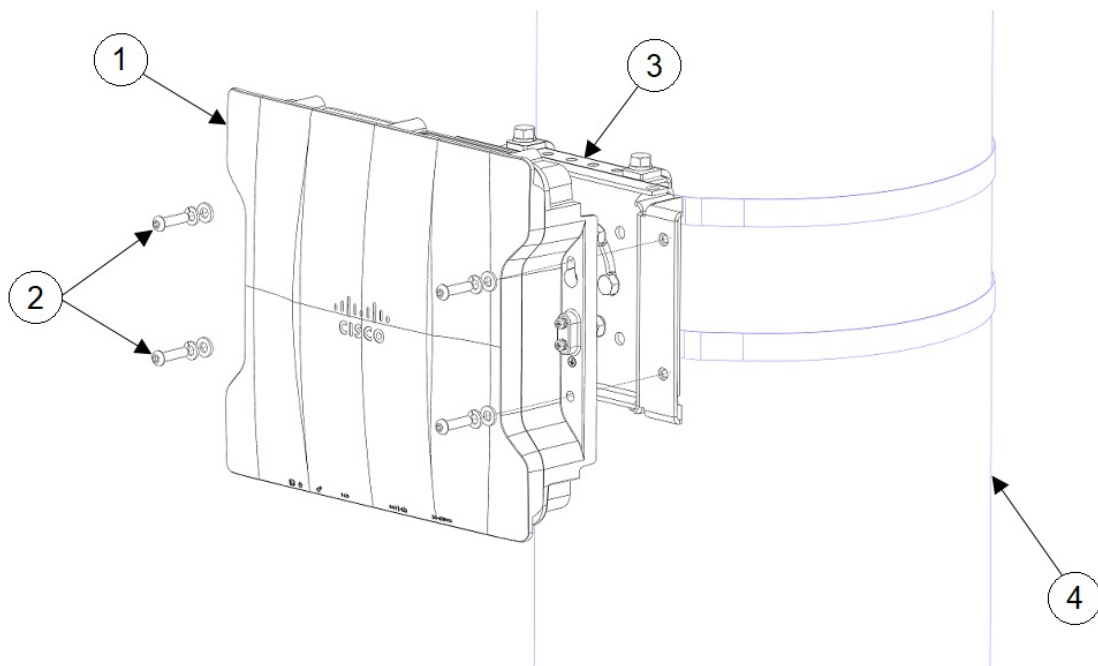
Figure 6: Access Point Installed in the Mounting Bracket
